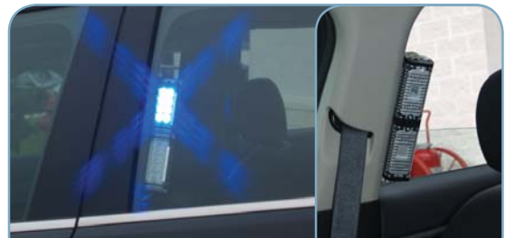
Predator 2™ Dual lights mounted in the interior on an undercover Chevrolet Caprice offer discrete side warning.
